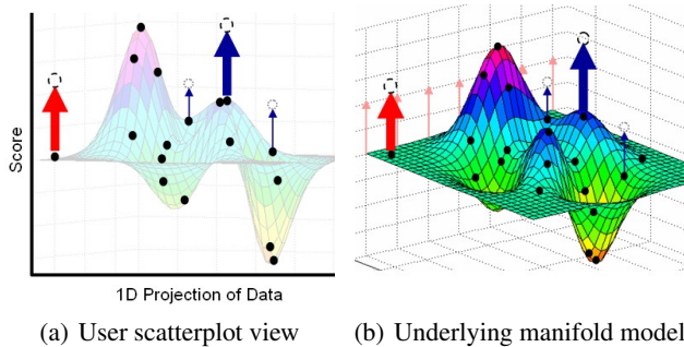
Figure 2: Interactive learning of a model, showing the user dragging two points (large light red and dark blue arrows) and the effect on the other data points and underlying scoring function. The red adjustment has a large effect due to the (geometrical) importance of this point, while the blue adjustment affects only points on the local peak.
